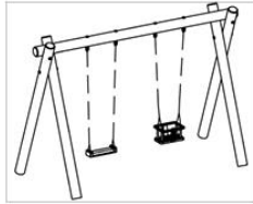
Twin Swing with Toddler Seat Age range: Nursery children Material: Timber and stainless steel Approximate size: 3.1m (L) x 1.9m (W) x 2.5m (H) Finishing: To manufacturer's specification
