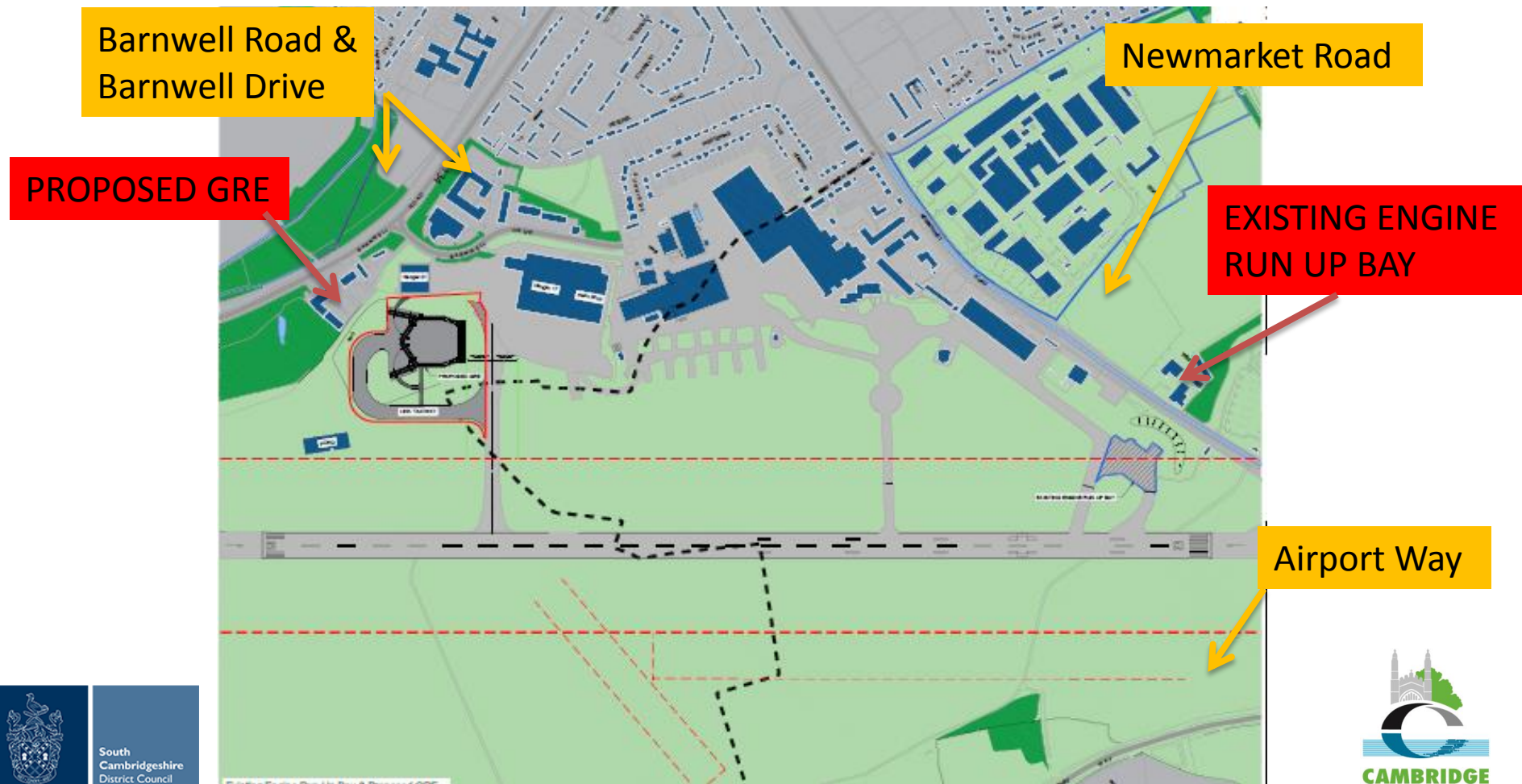
Location Plan
